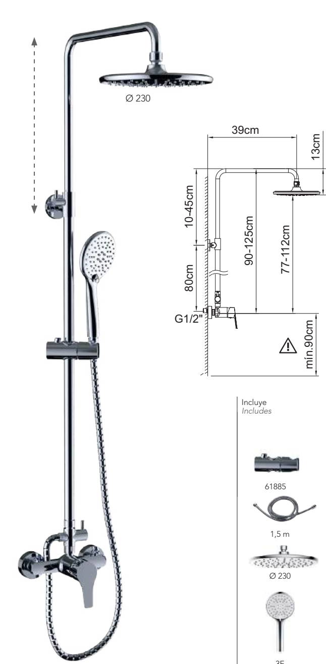
Conjunto de ducha monomando con barra extensible con soporte articulado deslizante. Single-lever shower set mixer with extendable bar with sliding articulated support.
