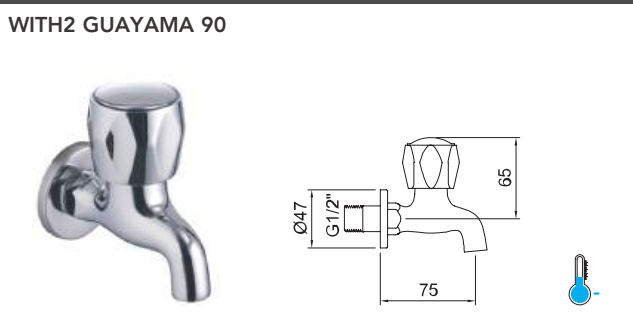
Grifo lavabo mural 1/2". Wall mounted basin tap 1/2".
