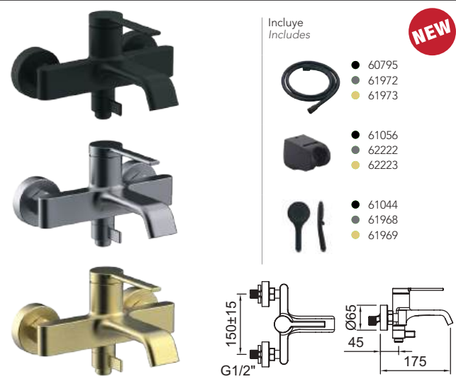
Baño- ducha monomando con aireador e inversor cerámico. Single-lever bath-shower mixer with aerator and ceramic diverter.
