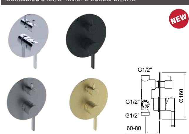
Ducha monomando empotrar 1/2". Concealed single-lever shower mixer 1/2".
