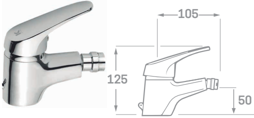
MONOMANDO BIDET Ref. 23204 € 35,00
