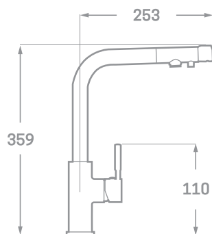
MONOMANDO FREGADERO OSMOSIS DESIGN ACABADO CROMO Ref. 23629
